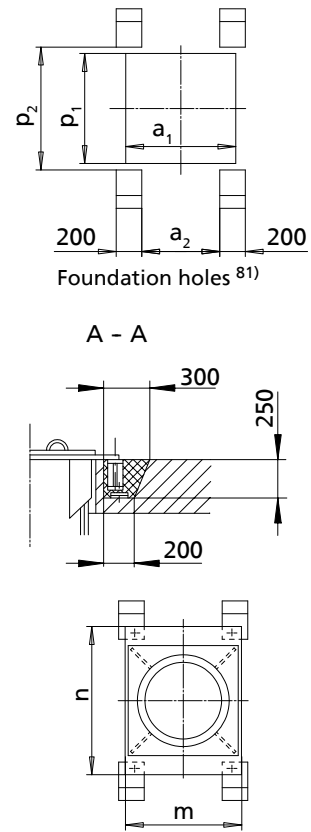
Detail X: support plate of the discharge tube Drawing without pump
