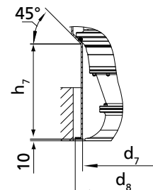
Detail Y: seating ring
