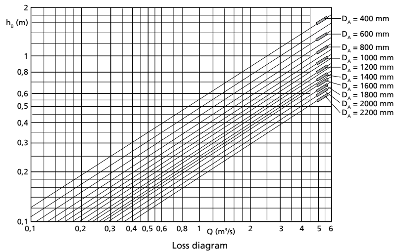
Loss diagram
