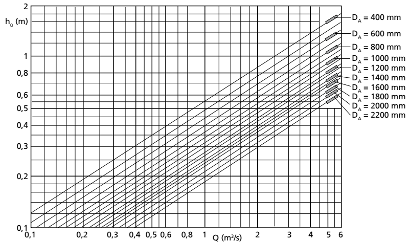
Loss diagram
