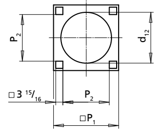
Foundation holes 8)
